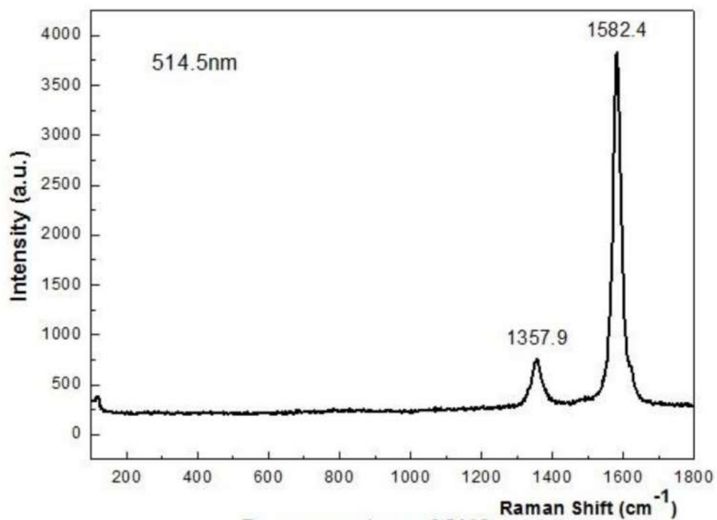
Raman spectrum
